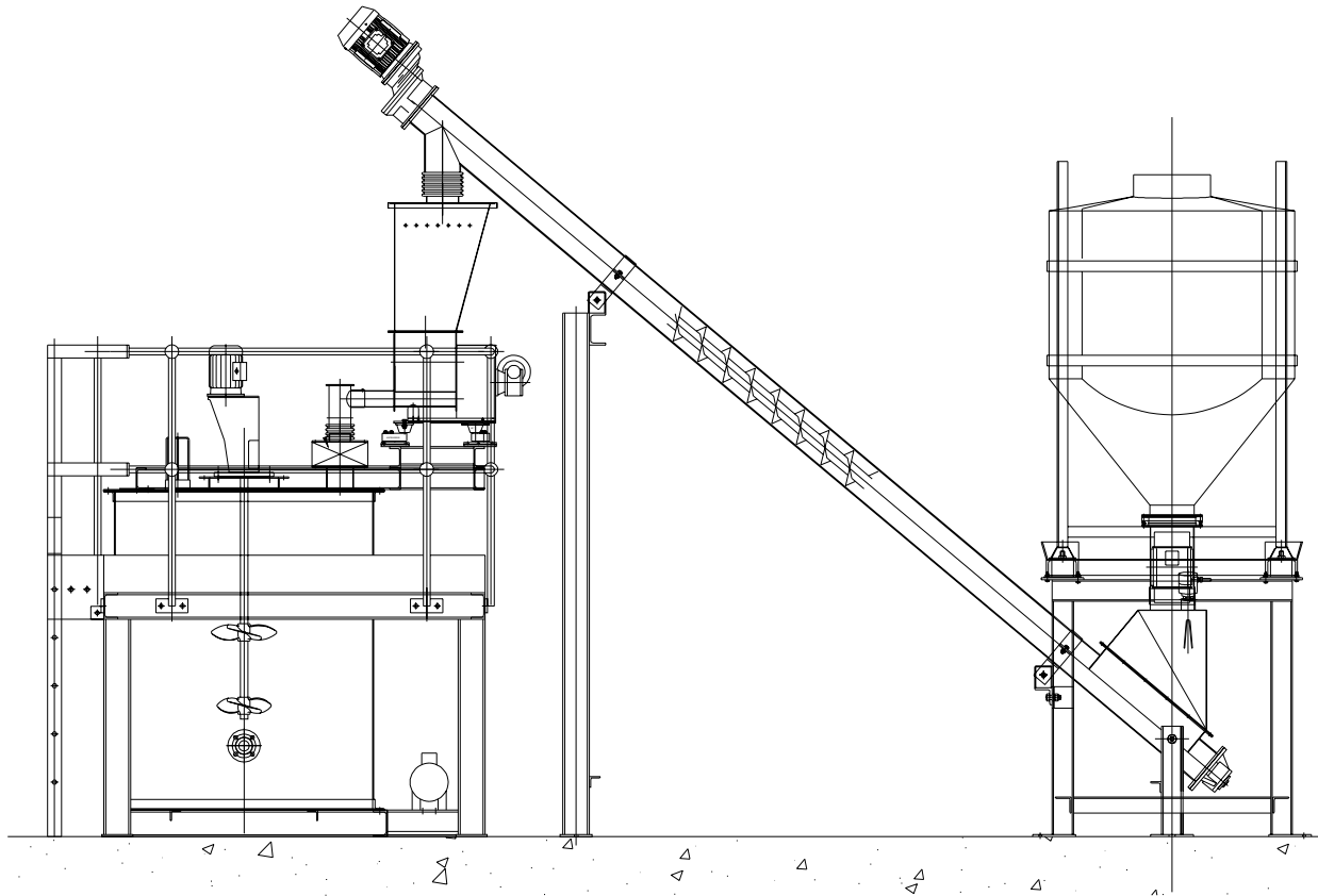
PAC Slurry Preparation Plant Installed 2003 - Contract Value £52,000 Client: Degremont & Northumbrian Water
